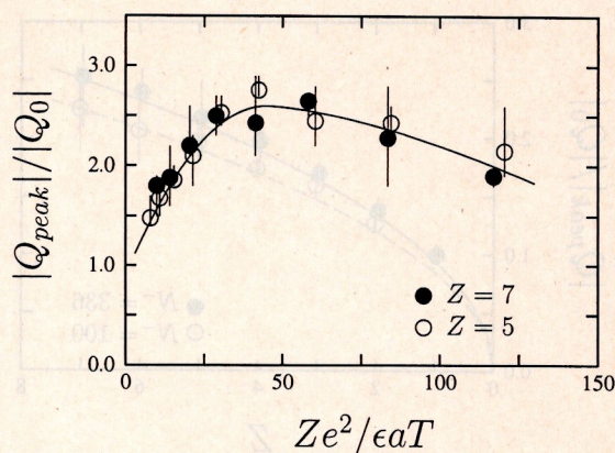
FIG. 6. Dependence of inverted charge on temperature is shown for counterions of different valence Z ; it is given by a master curve. The abscissa is the ratio of the Coulomb energy of the counterions to thermal energy, \Gamma_a = Ze^2/\epsilon aT . The radius of macroion is R_0 = 3a , and the number of coions is kept nearly the same, N^- \sim 335 and 336 for Z=5 and 7, respectively.
