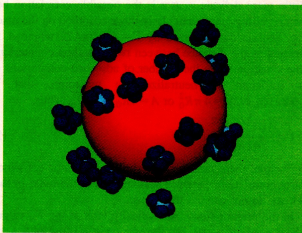
FIG. 3. (Color) The bird's-eye view of the screening atmosphere within 3a from a "large" macroion, at t=4000\omega_p^{-1} for the run of the macroion radius R_0=8a . Other simulation parameters are the same as those of Fig. 1, except that the temperature is adjusted to keep the quantity Ze^2/\epsilon R_0T the same as in Fig. 1. It means that \Gamma , Eq. (5), is the same here and in Fig. 1, while \Gamma_a is greater here by a factor of 8/3 than in Fig. 1. Accordingly, stronger binding of monovalent coions (dark blue) to multivalent counterions (light blue) is observed, and adsorbed counterions are less strongly correlated.
