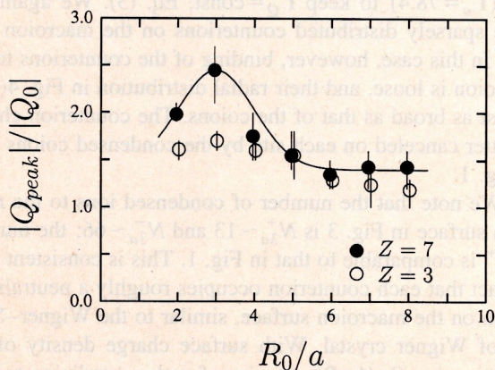
FIG. 5. Dependence of the inverted charge on the radius of macroion R_0 is shown for the counterions with the valence Z=3 and 7. The charge of the macroion is Q_0 = -28e ; the number of coions N^- = 335 (or 336) corresponds to the density n^- \sim 1 \times 10^{-2} a^{-3} . The ordinate is the maximum of the integrated charge Q_{\text{peak}} = \max(Q(r)) [Eq. (9)], normalized by the macroion charge |Q_0| . Each data point is an average of three runs, and a vertical bar shows the range of time variations and deviations among the runs.
