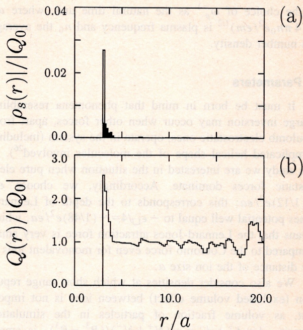
FIG. 2. Charge inversion under the "standard parameters," as in Fig. 1. (a) The radial distribution function of the charge \rho_s(r) [Eq. (8)] of counterions (open bars) and that of coions (shaded bars) as a function of the distance r from the macroion center. (b) The integrated charge distribution Q(r) of counterions plus coions [Eq. (9)]. The portion Q(r)/|Q_0|>1 corresponds to charge inversion. Comparatively large fluctuations near the wall is mainly due to the volume element 4\pi r^2 .
