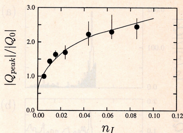
FIG. 9. Dependence of inverted charge on the ionic strength n_I = (Z^2 N^+ + N^-)/V , where V is the volume of the simulation domain. Charge neutrality of the system is maintained. The guide curve is n_I^{1/2} for n_I < 0.02/a^3 , and n_I for n_I > 0.05/a^3 . The macroion radius is R_0 = 3a , charge Q_0 = -28e , the valence of counterions Z = 7 , and \Gamma_a = 4.2Z = 29.4 .
